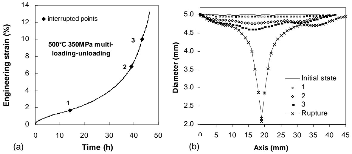
Fig. 2: Interrupted creep test performed at 500°C and 350MPa, (a) creep curve, (b) specimen diameter along axis measured at each interruption.
