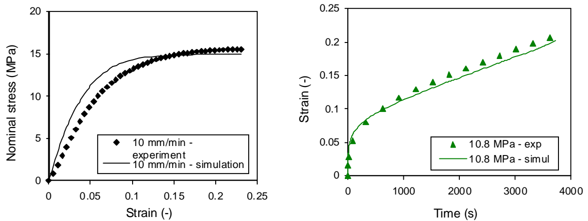
Figure 4: Comparison between experiment and simulation using a DDI model: a) tensile test at 10 mm/min, b) creep test à 10.8 MPa
