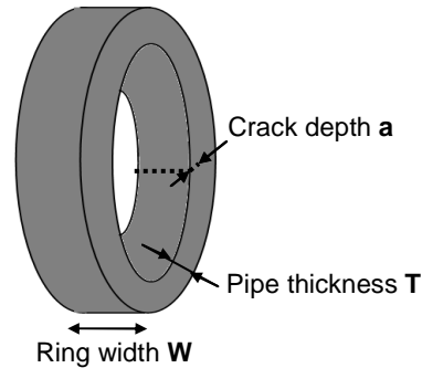
Figure 1: Precracked specimen dimensions
