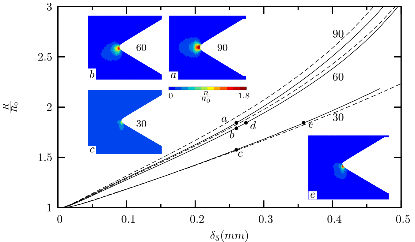
Figure 9: Arcan FE simulation: Rice and Tracey damage indicator ( R/R_0 ) vs. \delta_5 curves for different loading angles. Solid lines correspond to the L_N configuration while dashed lines correspond to T_N configuration. Maps show the damage indicator at various loading steps.
