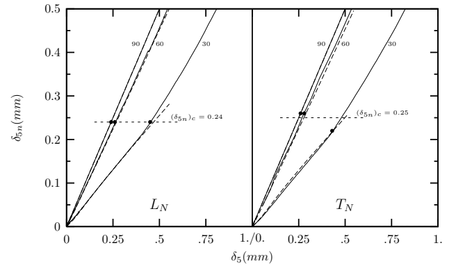
Figure 10: Arcan tests for T_N and L_N configurations: \delta_5 - \delta_{5n} curves. Dashed lines correspond to the FE simulation. Black dots represent experimental failure initiation (corresponding to ultimate force F_u ) for each case.
