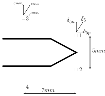
Figure 2: Specimens for mechanical testing.
