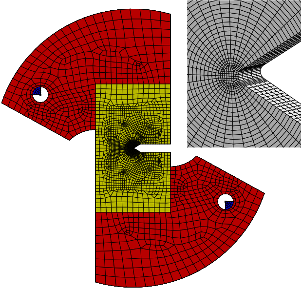
Figure 8: 3D Arcan mesh ( \beta = 30^\circ ) used for FE simulation.
