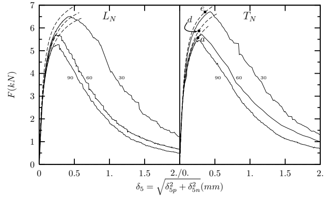
Figure 6: Arcan tests for T_N and L_N configurations: force— \delta_5 curves for different samples. Dashed lines correspond to the FE simulation. Black dots indicate the predicted fracture initiation using Rice and Tracey indicator (dots marked as a , d and e corresponds to damage plots in Fig. 9).
