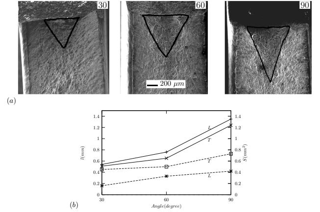
Figure 4: Fractographic examination: (a) Fracture surface SEM observations of Arcan sample ( L_N configuration), (b) Evolution of the triangular flat zone (length and surface) with respect to the loading angle \beta .
