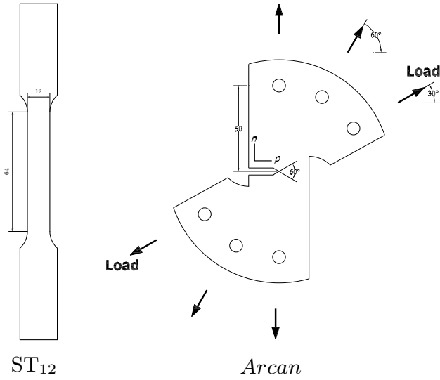
Figure 2: Specimens for mechanical testing.
