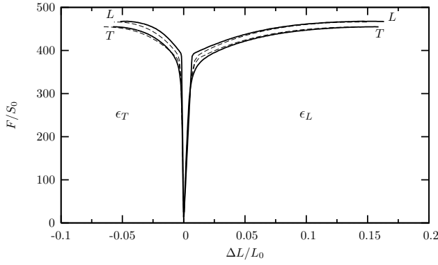
Figure 5: Tensile tests on ST_{12} along T and L directions: Nominal stress ( F/S_0 ) as a function of axial engineering strain ( \epsilon_L ) or long transverse engineering strain ( \epsilon_T ). Dashed lines correspond to the FE simulation with the optimized coefficients presented on Table 4 and Table 5.
