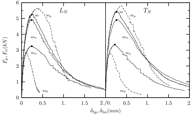
Figure 7: Arcan tests for T_N and L_N configurations: force— \delta_5 curves projected along normal and parallel axes for different samples. Black dots indicate the positions of the ultimate Force F_u , Local displacement \delta_{5n} for each case as reported on Table 3.
