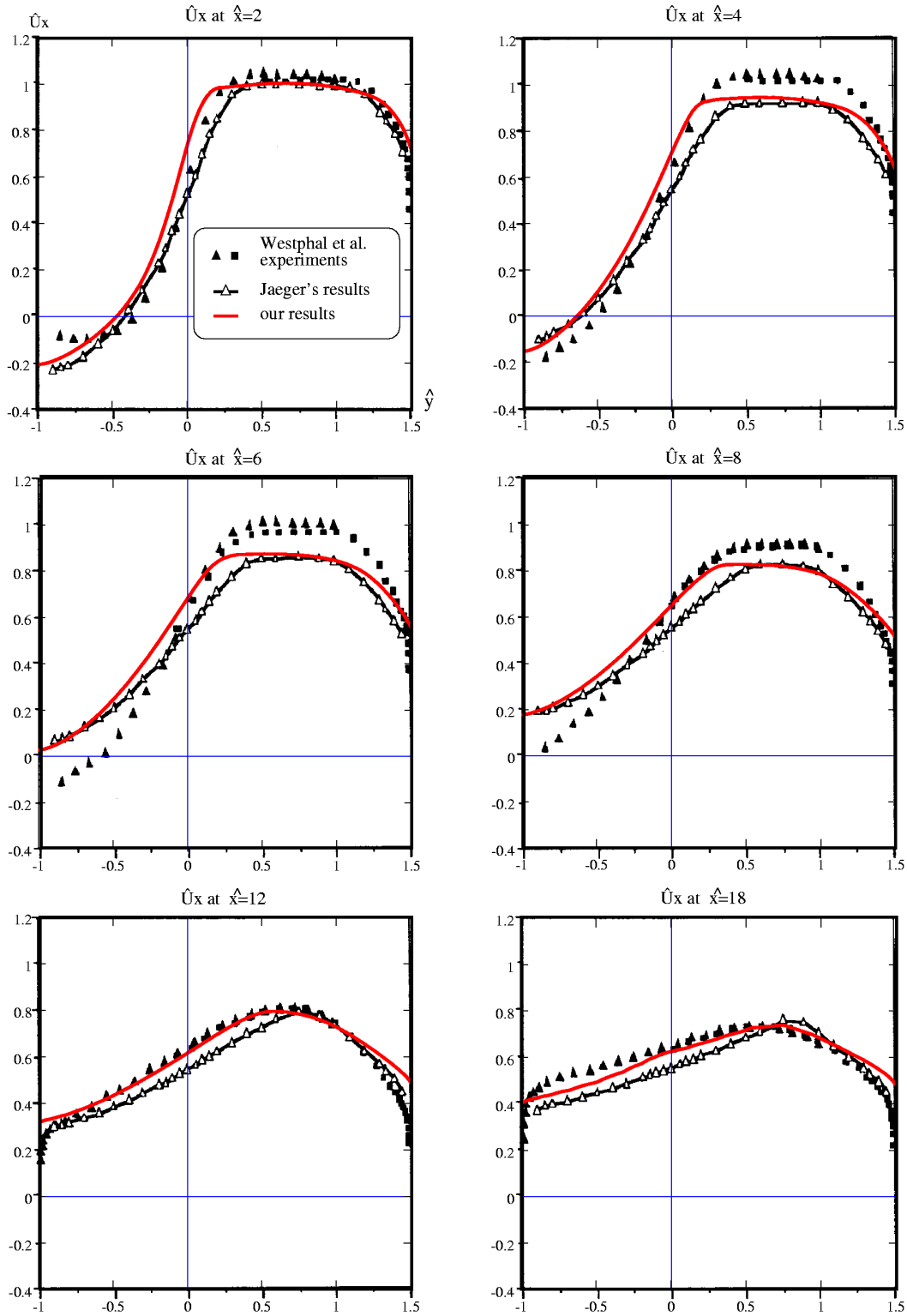
Figure 7: BFS test. Axial velocity profile in different transverse sections located at various horizontal coordinates. On each graphic, the normalised horizontal velocity \hat{U}_x = v_x / V_{av} is plotted versus the normalised vertical coordinate \hat{y} = y / H . The six graphics correspond to six transverse sections located at various normalised horizontal coordinates \hat{x} = x / H .
