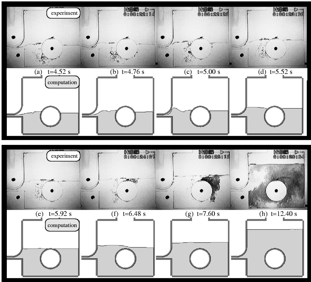
Figure 11b: Water model. Comparison between experimental flow and turbulent finite element computation.
