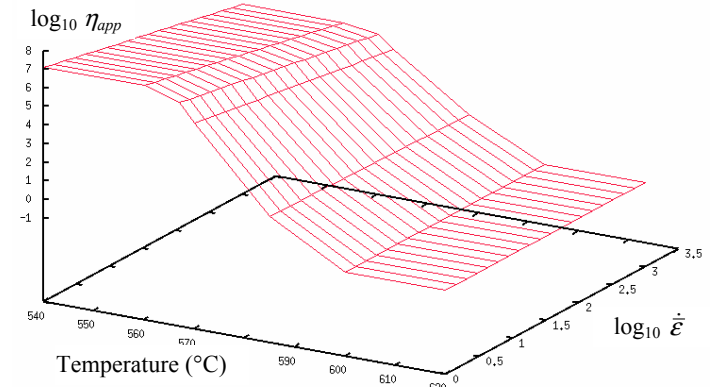
Figure 7. Variation of the apparent viscosity with respect to temperature and strain rate.
