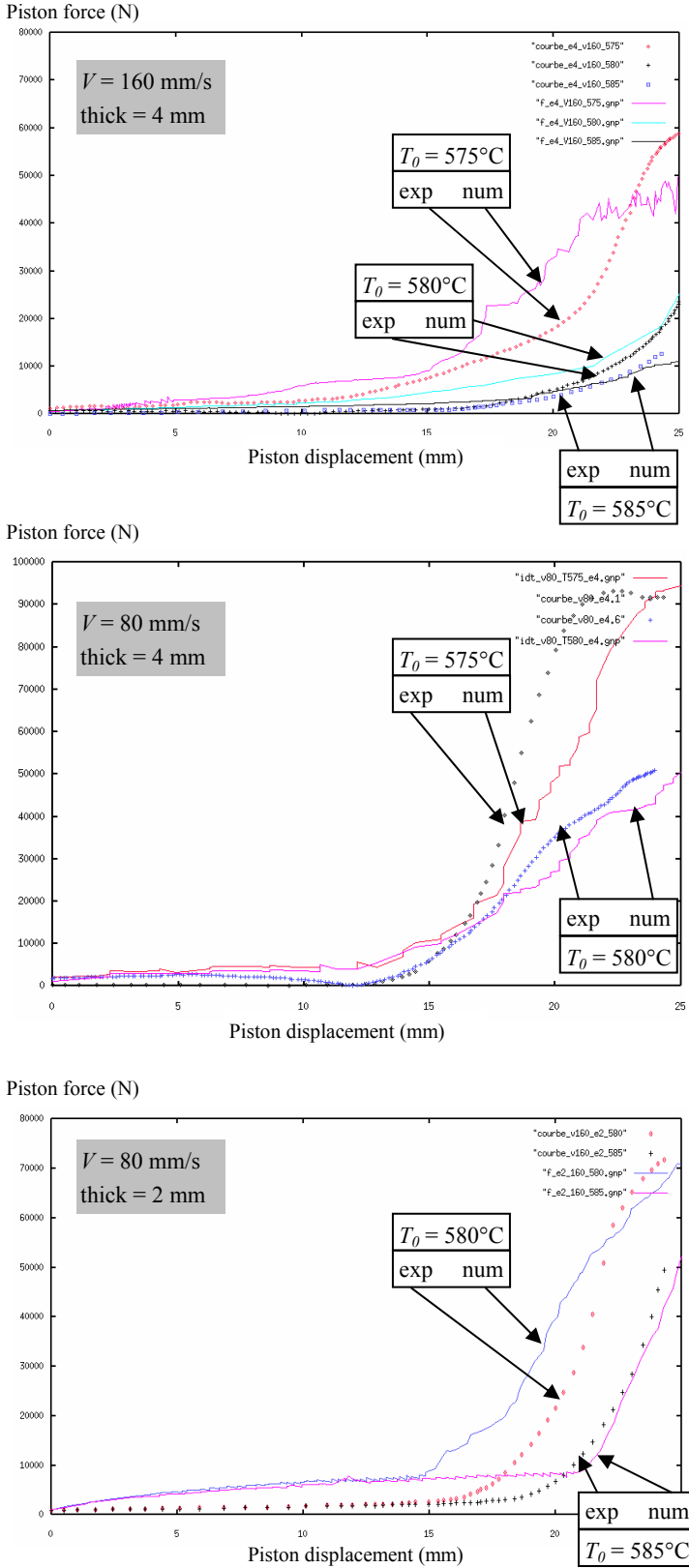
Figure 6. Comparison of measured injection forces and predicted ones.
