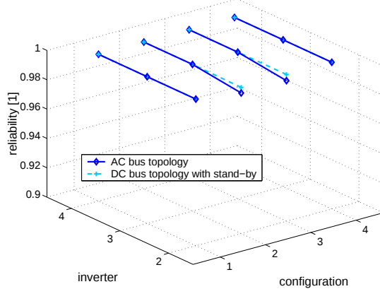
Figure 7: Reliability of the deferrable load (water pump)
