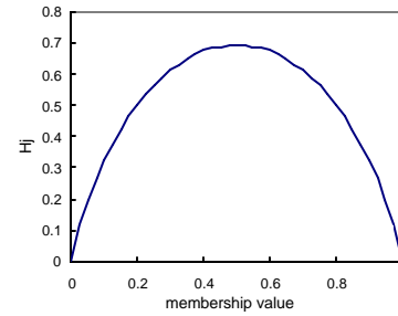
Figure 2: Entropy H_j of a fuzzy set as a function of the membership value \mathbf{m}(x) .
