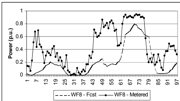
Figure 13: Wind forecast vs actual metered output for one wind farm for period 4 Sep 2001 to 8 Sep 2001.
