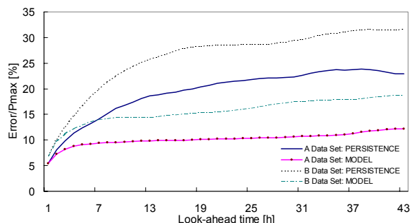
Figure 10: Performance of ARMINES model for a wind farm in Ireland
