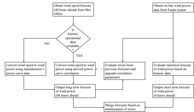
Figure 3: Diagrammatic flow chart of the RAL Meteo Wind Power Forecasting software
