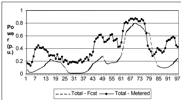
Figure 12: Total wind forecast vs Actual metered output for period 4 Sep 2001 to 8 Sep 2001.
