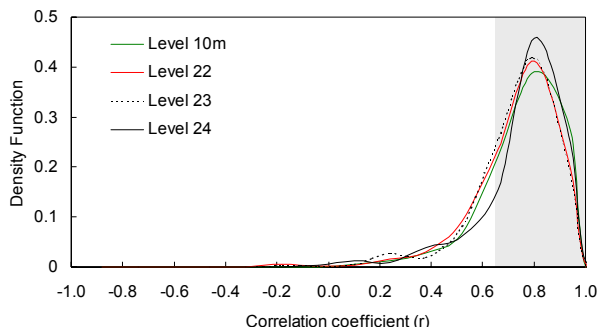
Figure 8: Distribution of correlation coefficient r(100) between Hirlam wind speed forecasts and measured wind park power.
