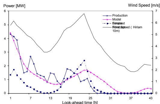
Figure 9: Comparison with a simple model.
