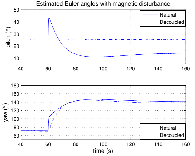
Fig. 4. Estimated pitch and yaw angles with magnetic disturbance
