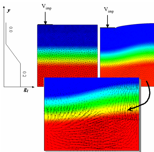
FIGURE 4. Redistribuition of the liquid inside a semi-solid domain with an initial fraction distribution.
