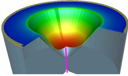
FIGURE 2. Conical geometry of the test with the deformed sheet and its strain distribution, as calculated by FORGE2® in axisymmetric 2D conditions. In reality, the sheet is formed upwards and the height sensor is pushed upwards.
