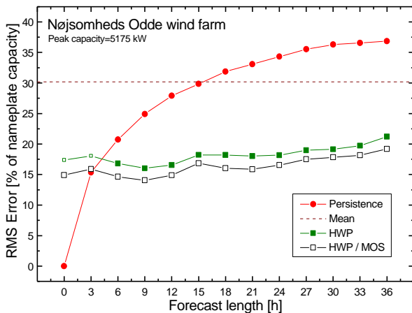
Figure 1: Root Mean Square (RMS) error for different forecast lengths and different prediction methods. The wind farm is the old Nøjsomheds Odde farm (before repowering) with an installed capacity of 5175 kW. HWP/MOS refers to the HWP approach (HIRLAM/WAsP/Park, nowadays called Prediktor) coupled with a MOS model (Model Output Statistics).
