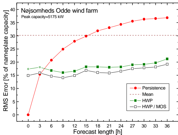
Figure 1: Root Mean Square (RMS) error for different forecast lengths and different prediction methods. The wind farm is the old Nøjsomheds Odde farm (before repowering) with an installed capacity of 5175 kW. HWP/MOS refers to the HWP approach (HIRLAM/WAsP/Park, nowadays called Prediktor) coupled with a MOS model (Model Output Statistics).
