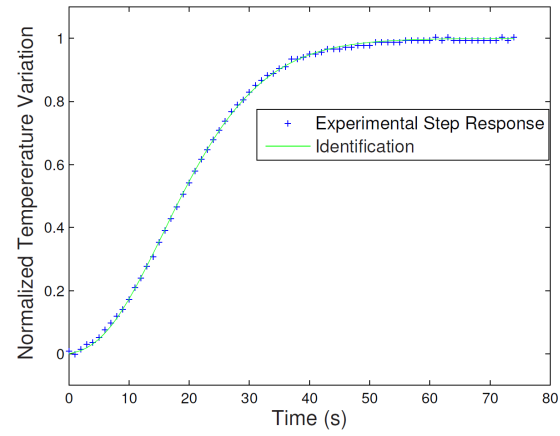
Fig. 3. Experimental data versus the DOC model
