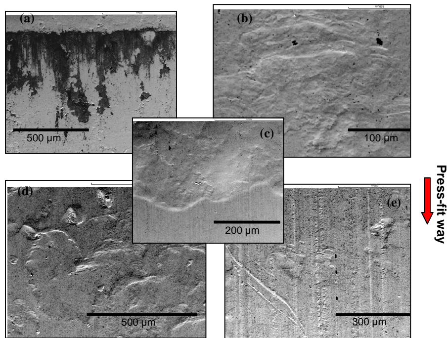
Figure 3 : SEM observation of rubbed polymer coating ; backscattered electron analysis, topographic mode – (a) :steel and phosphate show at surface of collar entry (complete wear of epoxy) – (b) : surface damage in the pushed-back epoxy area (before the “roll”) – (c) : “epoxy roll” (transition between sheared and rubbed epoxy coating areas) – (d) : after the roll: epoxy damage by wrenching of particles – (e) : after the roll: epoxy light superficial damage mainly by scratching
