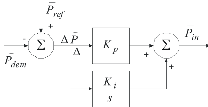
Figure 2b: Load following control system model
