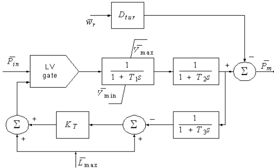
Fig. 3: Turbine model
