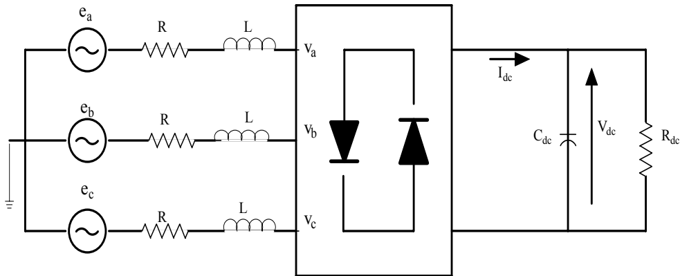
Figure 4: Circuit diagram of three-phase VSC
