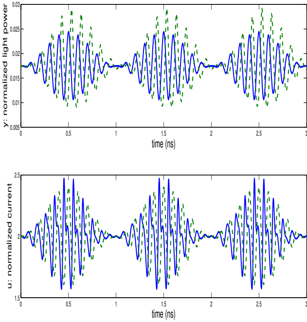
Fig. 1. Input current modulations with \epsilon(t) given by (4): the solid curve corresponds to the response of the diode when u is related to y = \bar{y}(1 + \epsilon(t)\cos(\omega t)) via (3); dashed line corresponds to the response of the diode when u = 1 + \left(1 + \frac{\tau_n}{\tau_c}\right)\bar{y}(1 + \epsilon(t)\cos(\omega t)) (static model).
