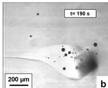
Figure 3: Advanced step of dissolution of cellulose xanthate in NaOH 8%-water under flow (shear rate – about 20 \text{s}^{-1} ) observed with the counter-rotating rheometer, at two successive dissolution time periods (a) 150 s, (b) 190 s. An increasing number of fibres dissolve and the highly viscous phase disperses into the solvent in the form of filaments
