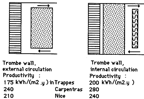
Fig. 7. Comparison of various solar walls
