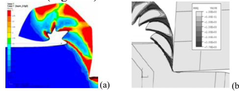
FIGURE 7. Strain distribution for present (a) and Bäker (b) models. The scale has been cut to 3.0.
