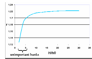
Fig. 8. Spread height r as a function of the bank - h_0=0,25\text{mm} ; R=125\text{mm} ; U=1,5\text{m/min} ; K=3000\text{Pa.s}^m ; m=0,62
