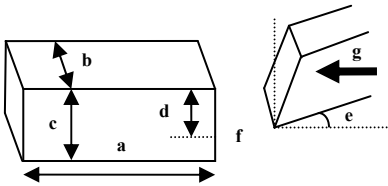
Figure 1: High speed orthogonal cutting test configuration.
