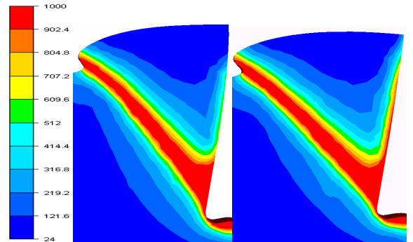
Figure 6: Temperature distribution ( ^{\circ}\text{C} ) for \bar{m} = 0.4 at t = 448 ns (left) and \bar{m} = 0.8 at t = 502 ns (right)
