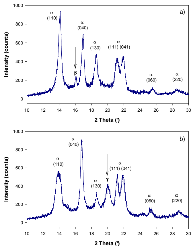
Fig. 5. WAXS patterns of: a) homopolymer, b) copolymer; after cooling-rate at 12^\circ\text{C}\cdot\text{min}^{-1} .
