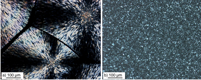
Fig. 1. Morphology development of : a) homopolymer PP3520 at 136 °C (110 μm-thick layer), b) copolymer PP7225 at 146 °C (12 μm-thick layer).
