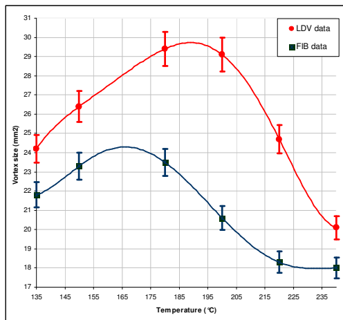
Fig. 6. Dependence of the vortex size on the temperature at m=0.3g/s , comparison between LDV and FIB data.
