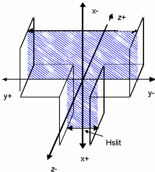
Fig. 3. Geometry of the flow cell and used coordinate system.
