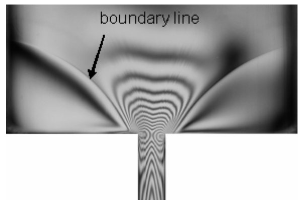
Fig. 5. Birefringence picture at T = 180^\circ\text{C} and m = 0.3 \text{ g/s} .
