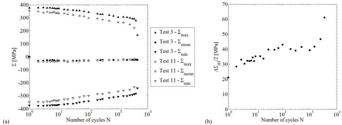
Fig. 3. (a) Evolution of maximum, minimum and mean stresses for test 3 and test 11 and (b) evolution of the difference between stress range of test 3 and stress range of test 11: \Delta\Sigma_{diff}(N) = \Delta\Sigma^{test\ 3}(N) - \Delta\Sigma^{test\ 11}(N) with \Delta\Sigma(N) = \Sigma_{max}(N) - \Sigma_{min}(N) for each test.
