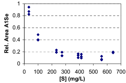
Fig. 11 : Relative area of A1Se-Se mode of Raman spectra as a function of the sulfur concentration
