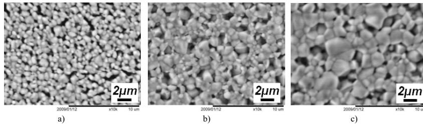
Fig. 1 : SEM top-view micrographs of \text{CuIn}(\text{S,Se})_2 absorbers annealed at a) 550°C, b) 600°C, c) 650°C maximum temperature after cyanide etching
