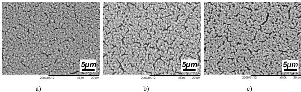
Fig. 3 : SEM top-view micrographs of \text{Cl}(\text{S,Se})_2 absorbers annealed with heating rate set at a) 1.8^\circ\text{C/s} , b) 2.4^\circ\text{C/s} , c) 8.8^\circ\text{C/s} after cyanide etching
