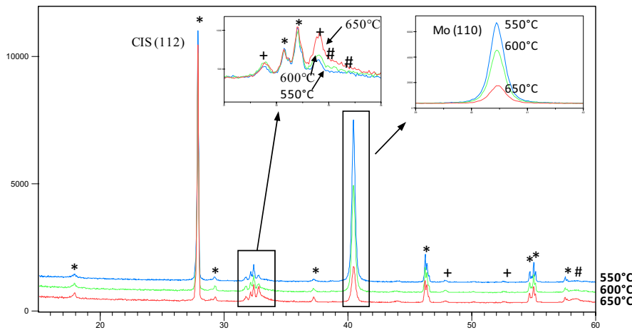
Fig. 2 :X-Ray diffractograms of samples annealed at 550, 600 and 650°C maximum temperature. The CIS phase is marked with asterisks, the \text{CuS} covellite with + signs and \text{Mo}(\text{S,Se})_2 with #
