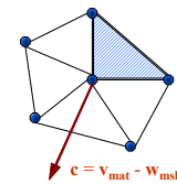
Figure 2: Upwind element
