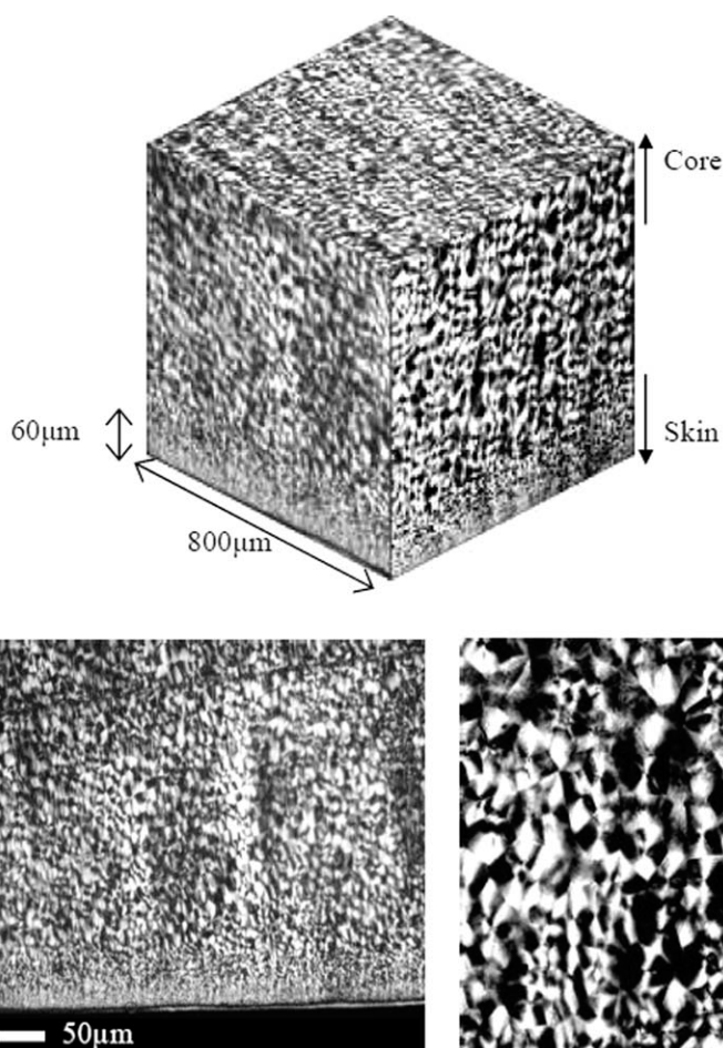
FIGURE 1 Optical microscope examinations of the size distribution of spherulites–Skin effect. (Adapted after [6])
