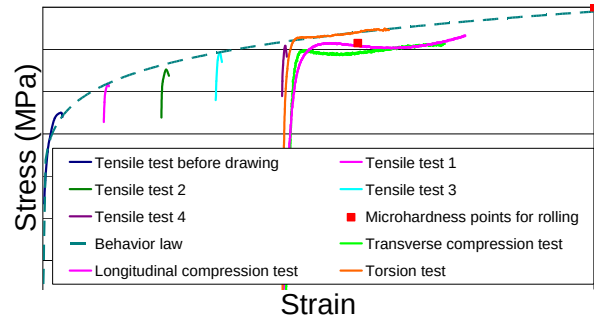
Figure 7: Strain-stress curves at all stages of the cold forming process (scales withdrawn for confidentiality)
