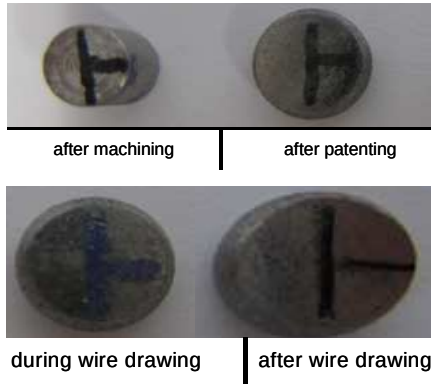
Figure 3: Compression tests in transverse direction highlight evolute anisotropy. Initial dimensions are H = 6 mm, R = 2.5 mm. Height reduction 43%. The horizontal bar of the T is the radial direction; the vertical bar is the drawing direction.
