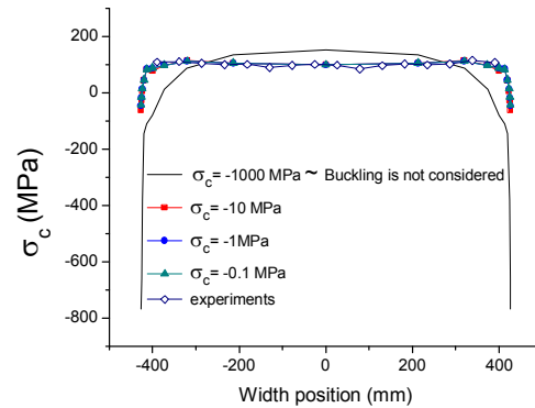
Figure 1: Comparison of stress profiles computed with and without accounting buckling, and measured in experiments (far away enough from the bite).
