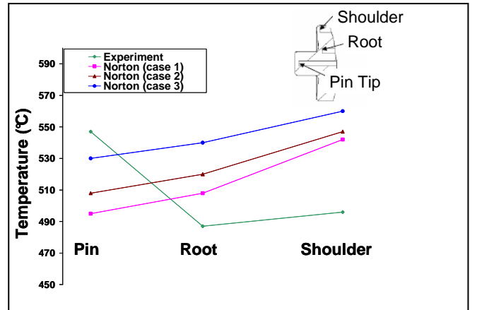
Figure 3: Comparison of calculated and measured temperatures at pin, root, and shoulder locations in the FSW tool with a Norton friction, using an Eulerian formulation
