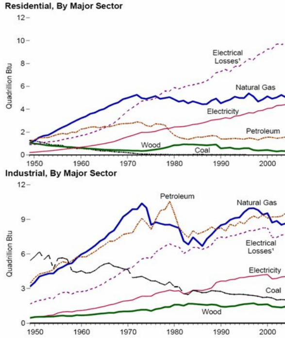
Figure 2: US energy consumption in the residential and commercial sector (up) and industry sector (down) from 1950 to 2005 [5].
