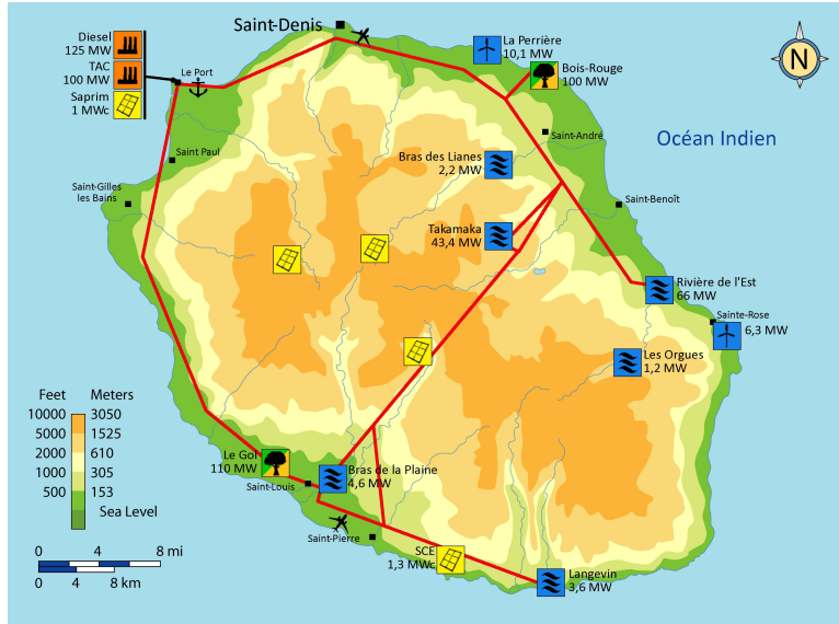
Figure 5: The power system of the Reunion Island [19].
