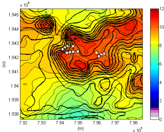
Figure 15: The same as Fig. 14 for the horizontal wind speed (m s -1 ) of the extreme simulations.
