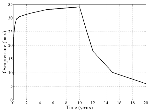
Figure 5: Hydromechanical simulations of the injection of CO 2 into the Dogger formation (from reference xvi ). The maximum overpressure is observed above the injection point at the reservoir-caprock limit. The injection is stopped after 10 years.
