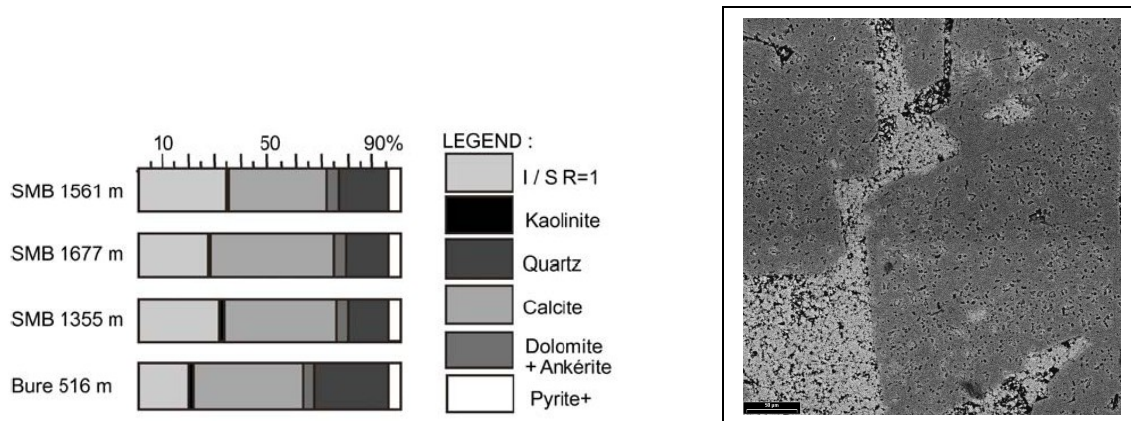
Figure 2: Example of analysis of two caprock faciès. Left: main mineral content of Callovo-Oxfordian argilites from the SMB and Bure area [xiv]. Right: SEM visualization of a dolomitic tight carbonate caprock, Comblanchien faciès [viii]. The thick black line indicates a scale of 50 \mu m.
