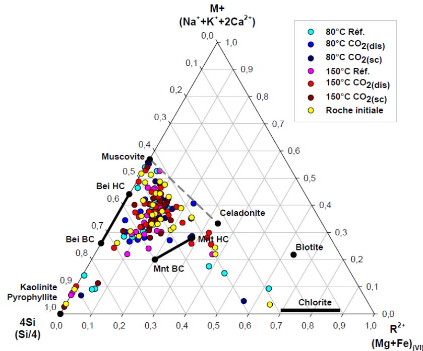
Figure 4: Triangular diagram summarizing the TEM mineralogical analysis of samples exposed to CO 2 at 150 bar during 6 months at 80 and 150°C. The dispersion of the points representing the rock before alteration is similar after CO 2 exposure (from reference xiv).
