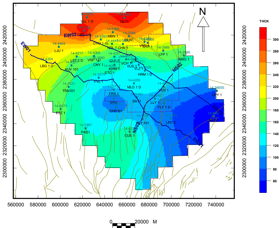
Figure 1 : Result of the interpolation between wells to determine the thickness of clayey formations above the Dogger formation (from reference viii). The right scale indicates the estimated thickness from 60 up to 300 m. The thick lines indicate the available seismic profiles. The SMB field is located approximately at the crossing of NS02 and EW02 seismic lines. The inset indicates the Picoref area.
