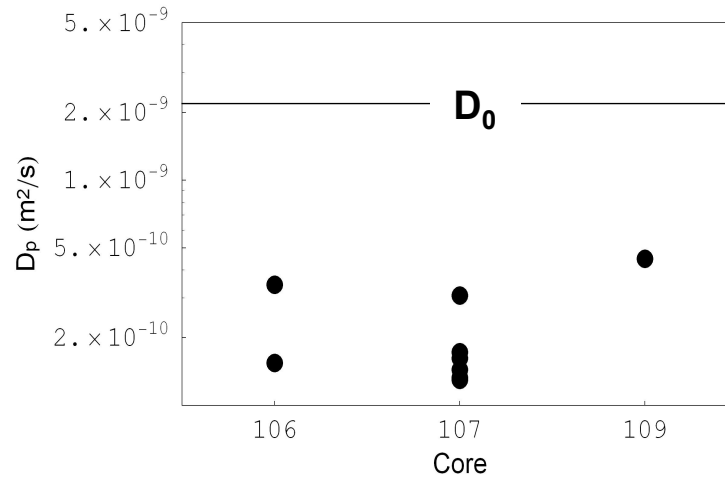
Figure 3: Pore water diffusivity measurements on three samples from the SMB field, transition zone, representing an upper limit for the diffusion of dissolved CO 2 , from reference ix. Porosity 6 %, permeability around 1 μ D.
