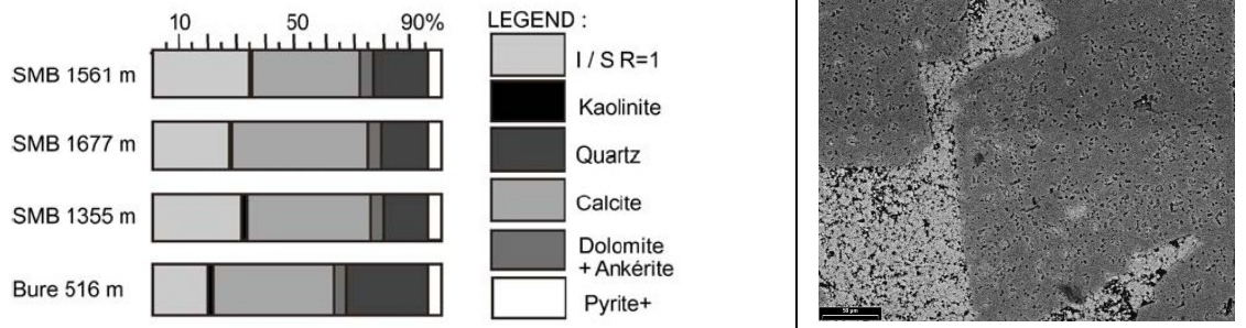
Figure 2: Example of analysis of two caprock faciès. Left: main mineral content of Callovo-Oxfordian argilites from the SMB and Bure area [xiv]. Right: SEM visualization of a dolomitic tight carbonate caprock, Comblanchien faciès [viii]. The thick black line indicates a scale of 50 \mu m.
