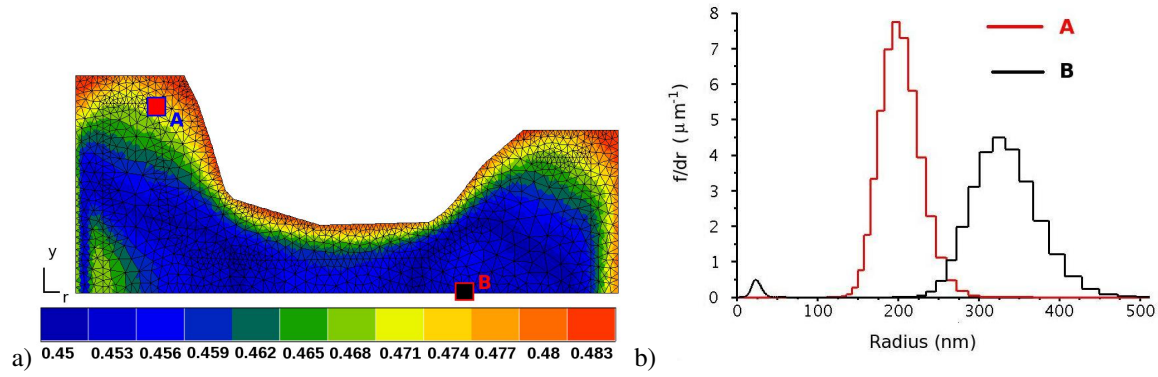
Figure 13: Volume fraction of \gamma' precipitates inside 1/2 disk during the quench. a) Contour of the \gamma' volume fraction, b) \gamma' size distribution for a point near the surface (A) and in the core of the disk (B) after treatment.
