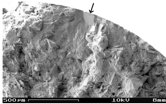
Figure 9: Fractography of a crack initiation of the specimen submitted to LCF test 3 with the supersolvus standard microstructure.
