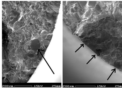
Figure 10: Fractographies of the crack initiations of the specimen submitted to incremental LCF test 4 with the supersolvus standard microstructure.
