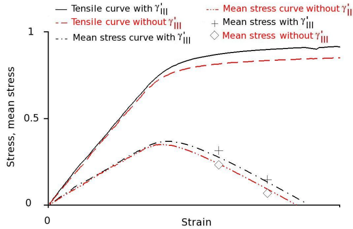
Figure 12: Relaxation of the mean stress. Continuous and dashed line: tension curve. Dashed-dotted line: \sigma - E\varepsilon/2 . Symbols: mean stress measured on the LCF tests 2 and 3.
