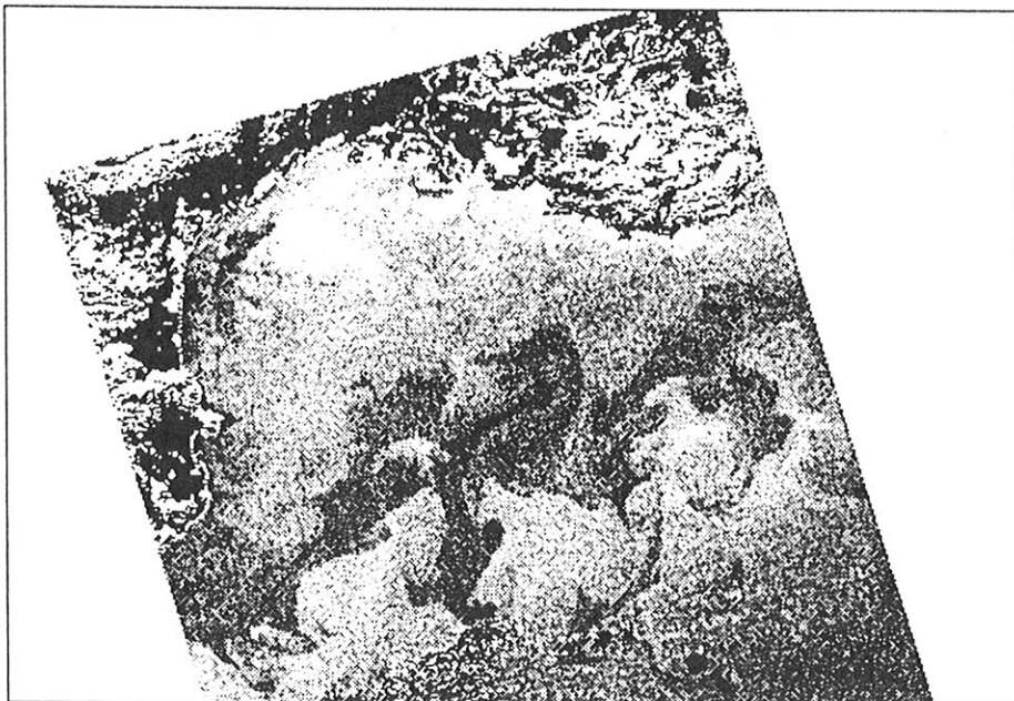
Figure 2 : Coastal Zone Color Scanner (CZCS) image of the northwestern Mediterranean Sea, February 1, 1981.
