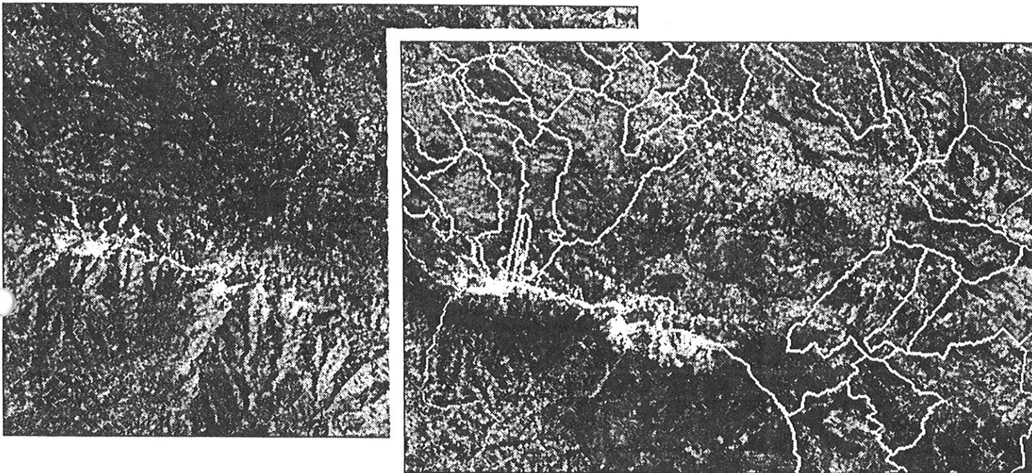
Figure 4 : Landsat/Multi-Spectral Scanner image of the region of Abruzzo (Italy). Two spectral images are presented. In one, district limits have been incrustated, which originate from digitized administrative maps. Processing of the spectral data provides a map related to the forest biomass available for energy conversion (in white and light grey).
