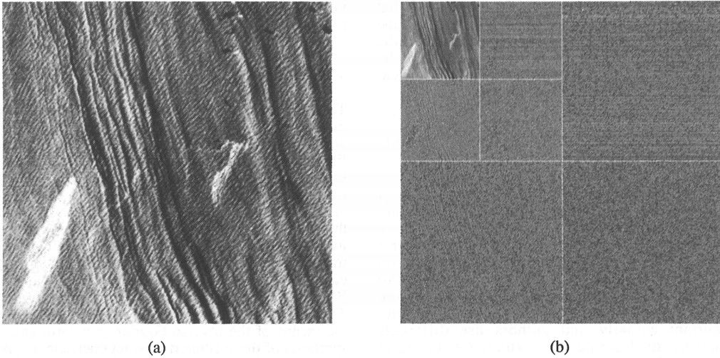
Figure 1: Multiresolution analysis of a SPOT image of the ocean. (a) Original image of the XS3 channel (near infrared). Resolution is 20 m. Sizes of image are 512x512. (b) decomposition into context image (resolution 80 m) and details images (characteristics lengths comprised between 20 and 40 m, and 40 and 80m) according to the scheme of Table 1.
