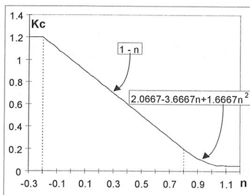
Figure 1. K_c^t = f(n^t)
