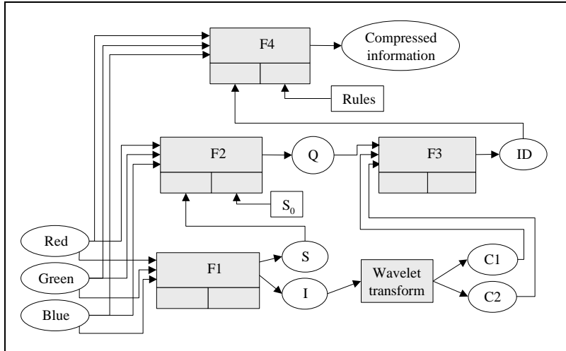
Figure 4.6. A scheme representing a data fusion process for data compression
