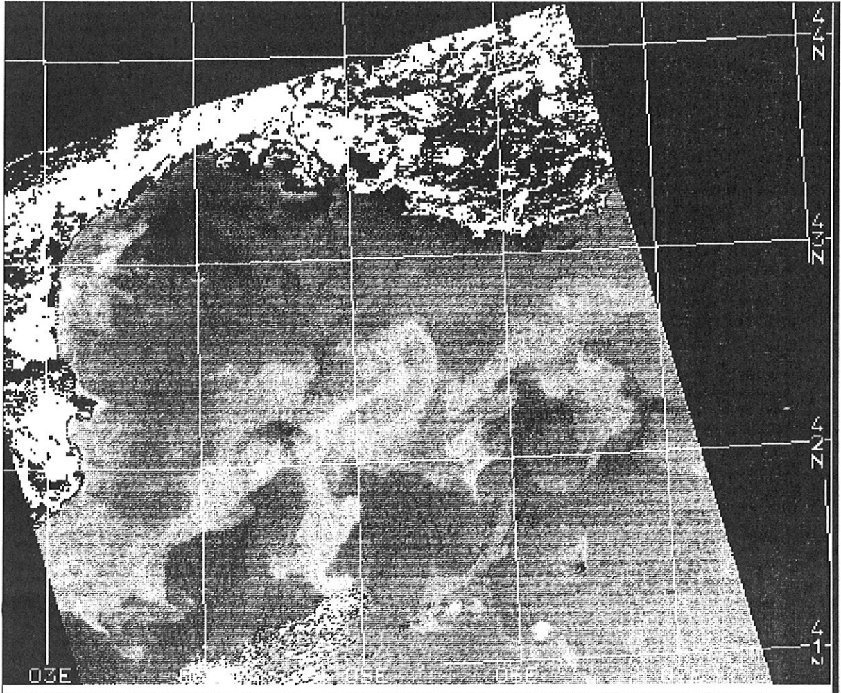
Fig. 5 Visible image of the gulf of Lion, observed in the blue channel by NIMBUS 7, on 1 February, 1981, at 1055 GMT. The darker the tone, the weaker the energy backscattered by the sea.
