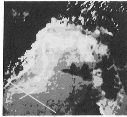
Fig. 1 (left): untreated image of the Liguro-Provencal basin from VHRR-NOAA 5 on 9 March 1978. The French and Italian Riviera coasts are visible. Cape of Corsica is seen black in the lower right.
