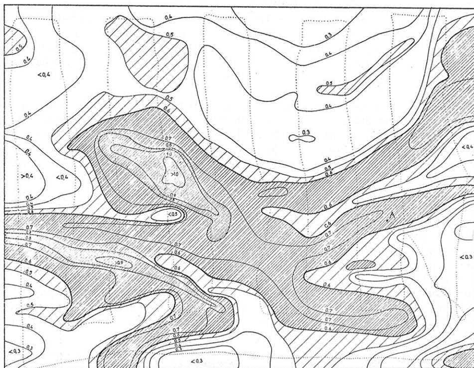
1 2 3 4 N nautical miles A position: 43° 20' 8N 7° 33' E ..... ship track — iseline of b ( 1/m ) 26-28/03/1980
