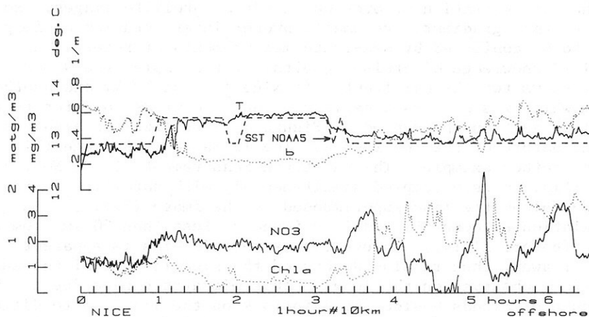
Fig. 3: Ship data of 7 March 1978 for pigments (Chla, \text{mg.m}^{-3} ), nitrate ( \text{NO}_3 , \text{mg.m}^{-3} ), temperature (T, deg. C) and total scattering coefficient (b, \text{m}^{-1} ) at the depth of 3 m, along the longer track on Fig. 2.
