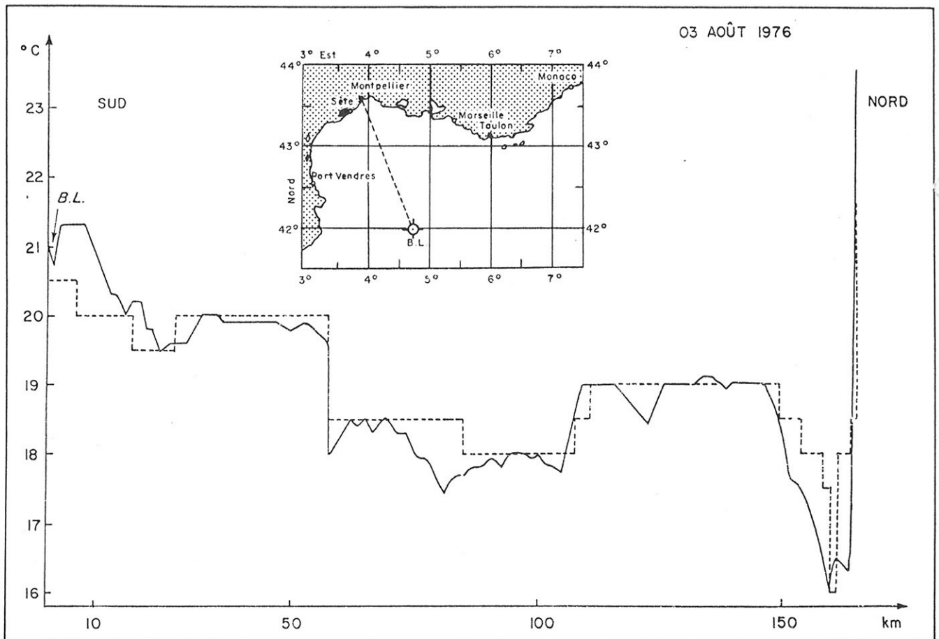
Figure 1 Sst profiles measured from "Aries" and "Noaa 4". Continuous line: "Aries" data (channel 1); dotted line: Vhrr data after the 1.5°C shift.
