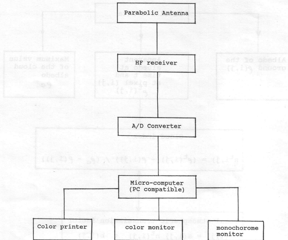
Fig. 2. Synoptic scheme of the Heliosat station.
