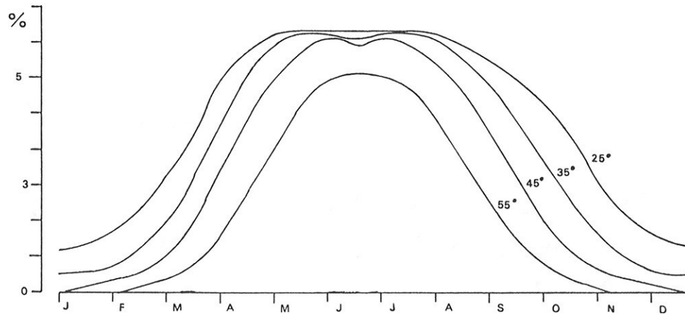
FIG. 1. Reflectance contrast observed on Landsat imagery for a non-absorbing atmosphere throughout the year for various latitudes: 25° N, 35° N, 45° N, and 55° N. See text for explanation.
