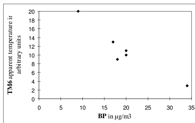
Figure 2. Correlation between black particulates for May 22, 1992 (BP, in µg/m 3 ) and apparent temperature observed by the satellite (in arbitrary units)
