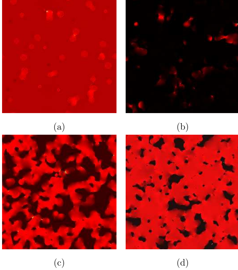
Fig. 13. 2D sections of the stress component \sigma_m in the random rigidly-reinforced medium, at various rigid inclusions concentrations f = 0.1 (a), 0.4 (b), 0.7 (c), 0.9 (d). A hydrostatic deformation \langle \varepsilon_m \rangle is applied. The color scale goes from black (smallest values) to white (highest values) with red and yellow in-between (color online).
