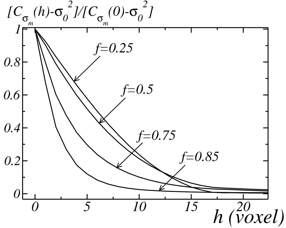
Fig. 7. Normalized covariance C_{\sigma_m}(h) of the mean component of the stress field \sigma_m as a function of the distance h (number of voxels), for a Boolean medium at various different porosities f = 0.25, 0.5, 0.75 and 0.85 . Along the x -axis, the length h is expressed in voxel units (the diameter of a sphere is 18 voxels). A hydrostatic load is applied as a macroscopic deformation \langle \varepsilon_m \rangle = 1 , on a 256^3 FFT grid.
